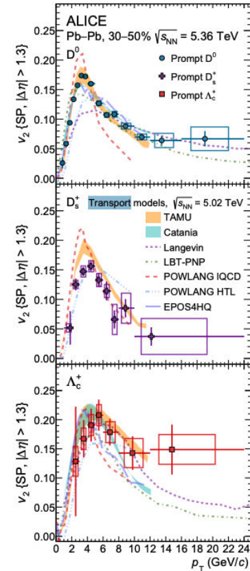
Figure 2: Elliptic flow of prompt D^0 (top), D_s^+ (middle), and \Lambda_c^+ (bottom) hadrons at midrapidity ( |y| < 0.8 ) in Pb–Pb collisions at \sqrt{s_{NN}} = 5.36 TeV in the 30–50% centrality class as a function of p_T . The data are compared with predictions from TAMU [78], Catania [43, 79], POWLANG [80, 81], LBT-PNP [44, 75], EPOS4HQ [76], and Langevin [82, 83] transport models at \sqrt{s_{NN}} = 5.02 TeV.
