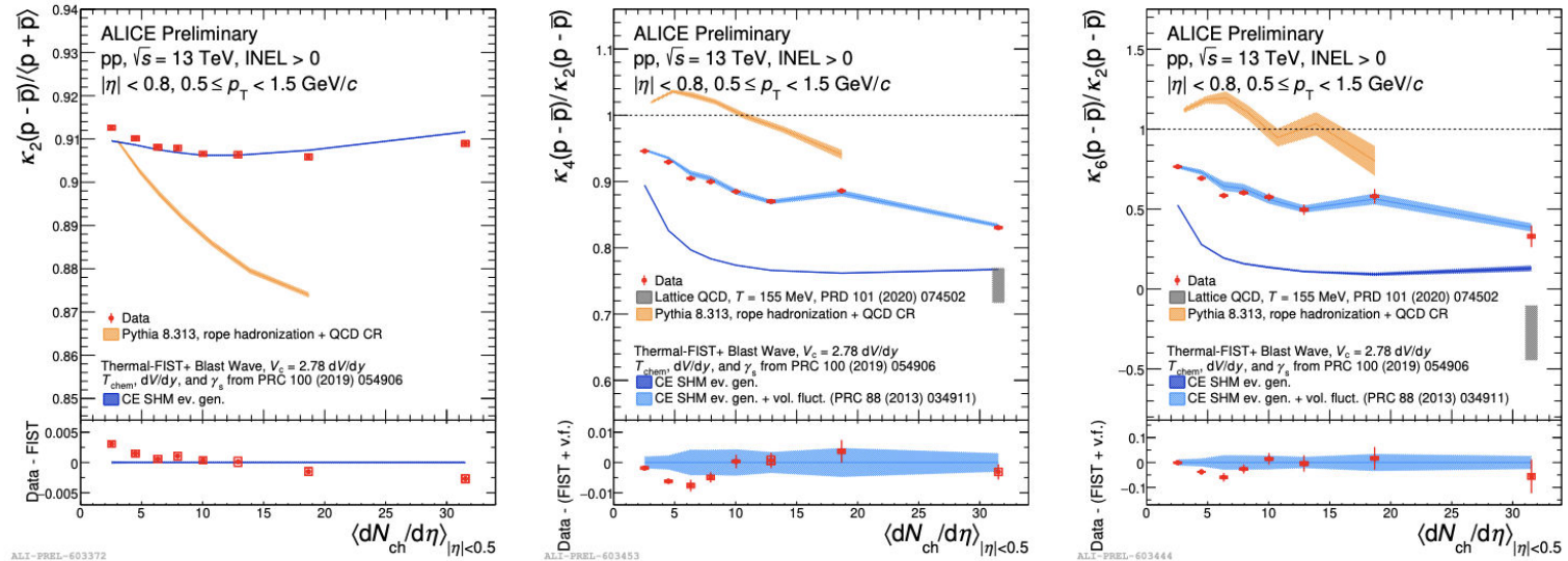
Figure 1: Net-proton number cumulant ratios \kappa_2(p - \bar{p})/\langle p + \bar{p} \rangle (left), \kappa_4(p - \bar{p})/\kappa_2(p - \bar{p}) (center) and \kappa_6(p - \bar{p})/\kappa_2(p - \bar{p}) (right) in pp collisions at 13 TeV as a function of the charged particle multiplicity density at midrapidity \langle dN_{ch}/d\eta \rangle_{|\eta|<0.5} .
