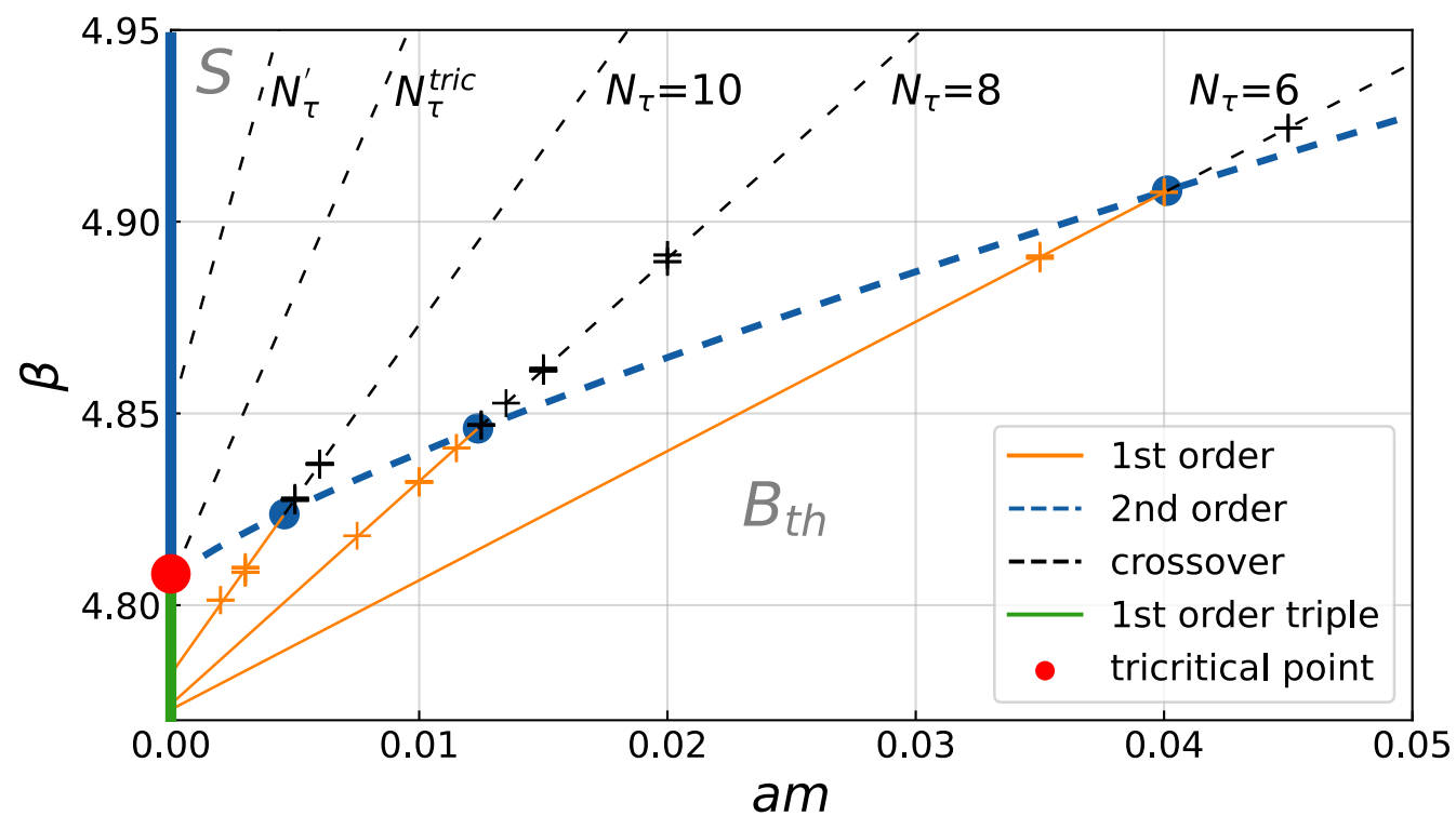
Thermal phase transition
